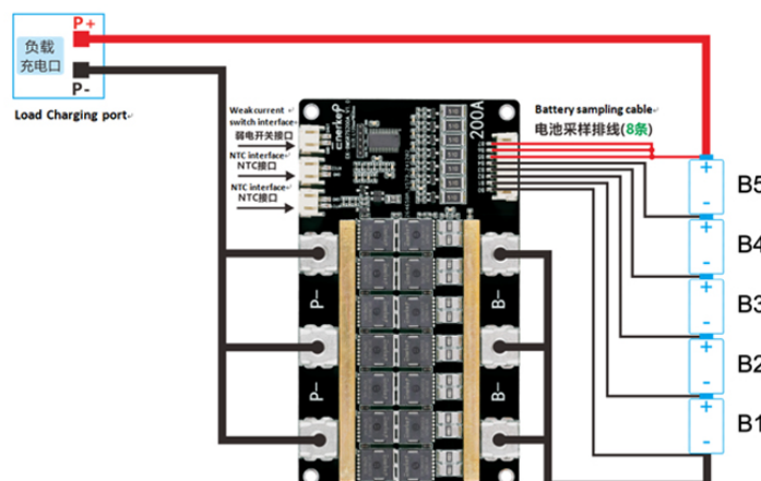
Wiring diagram of 6 battery strings
