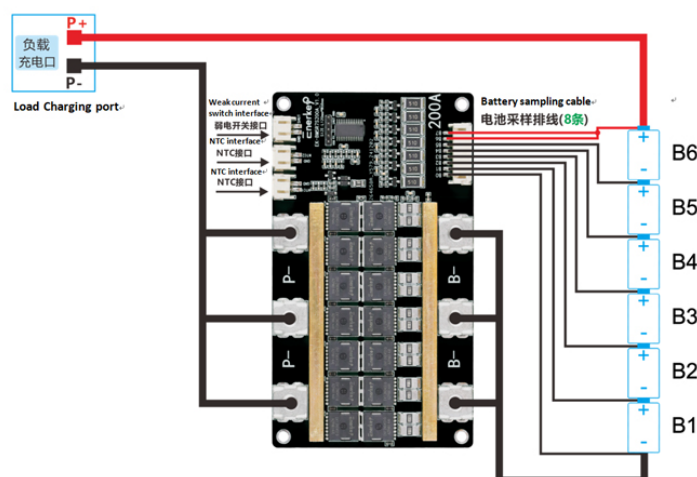
Wiring diagram of 7 battery strings
